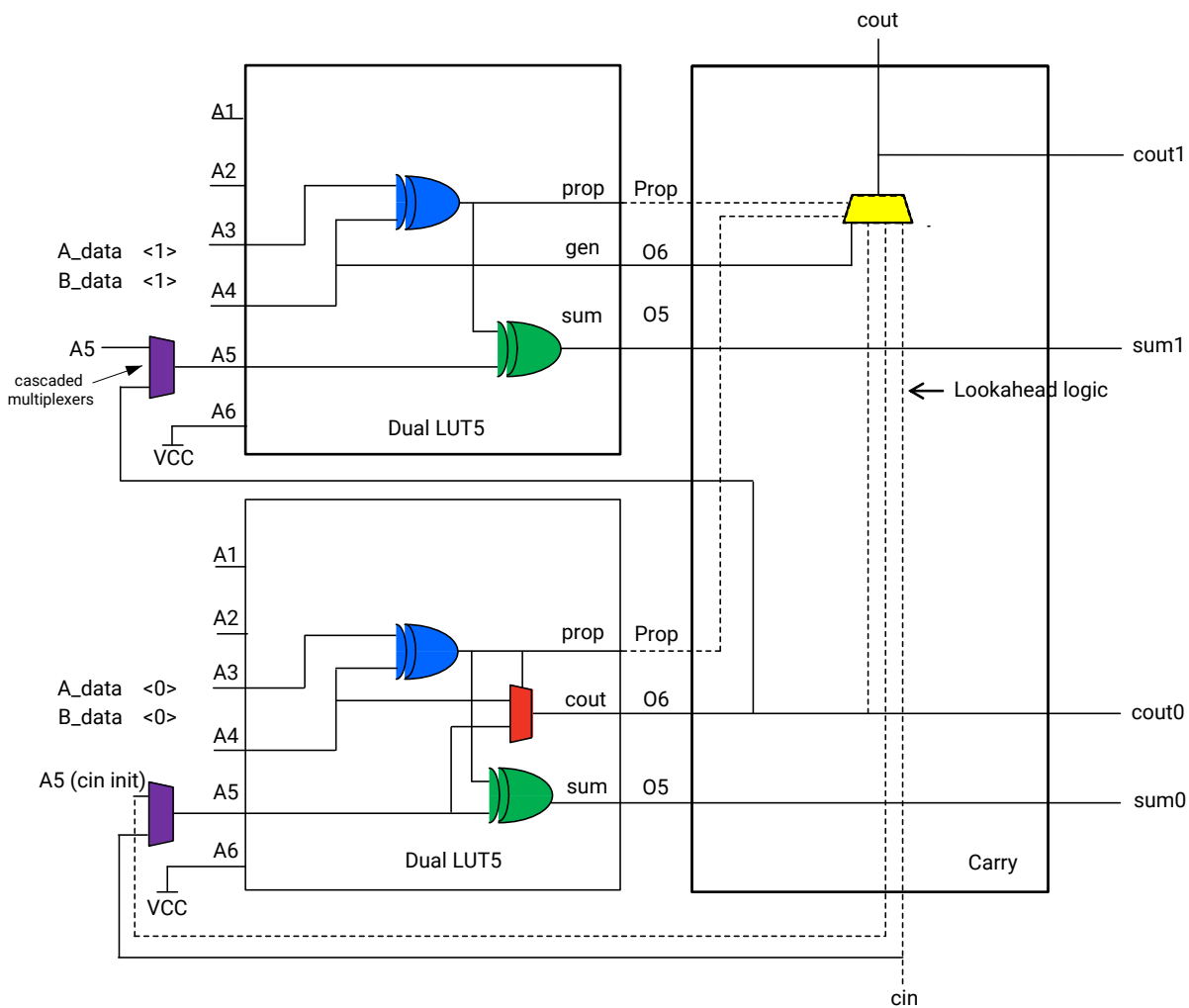
Figure 8: Carry Chain
