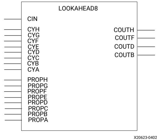
Figure 13: Carry Look-Ahead Logic Primitive
