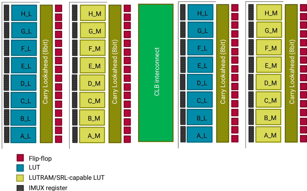
Figure 1: CLB Block Diagram
