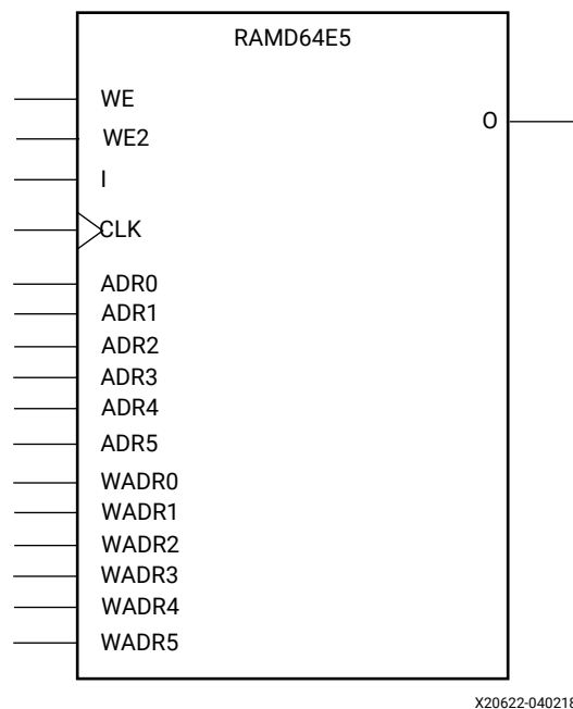
Figure 12: RAMD64E5 Distributed RAM Primitive (Dual-Port)
