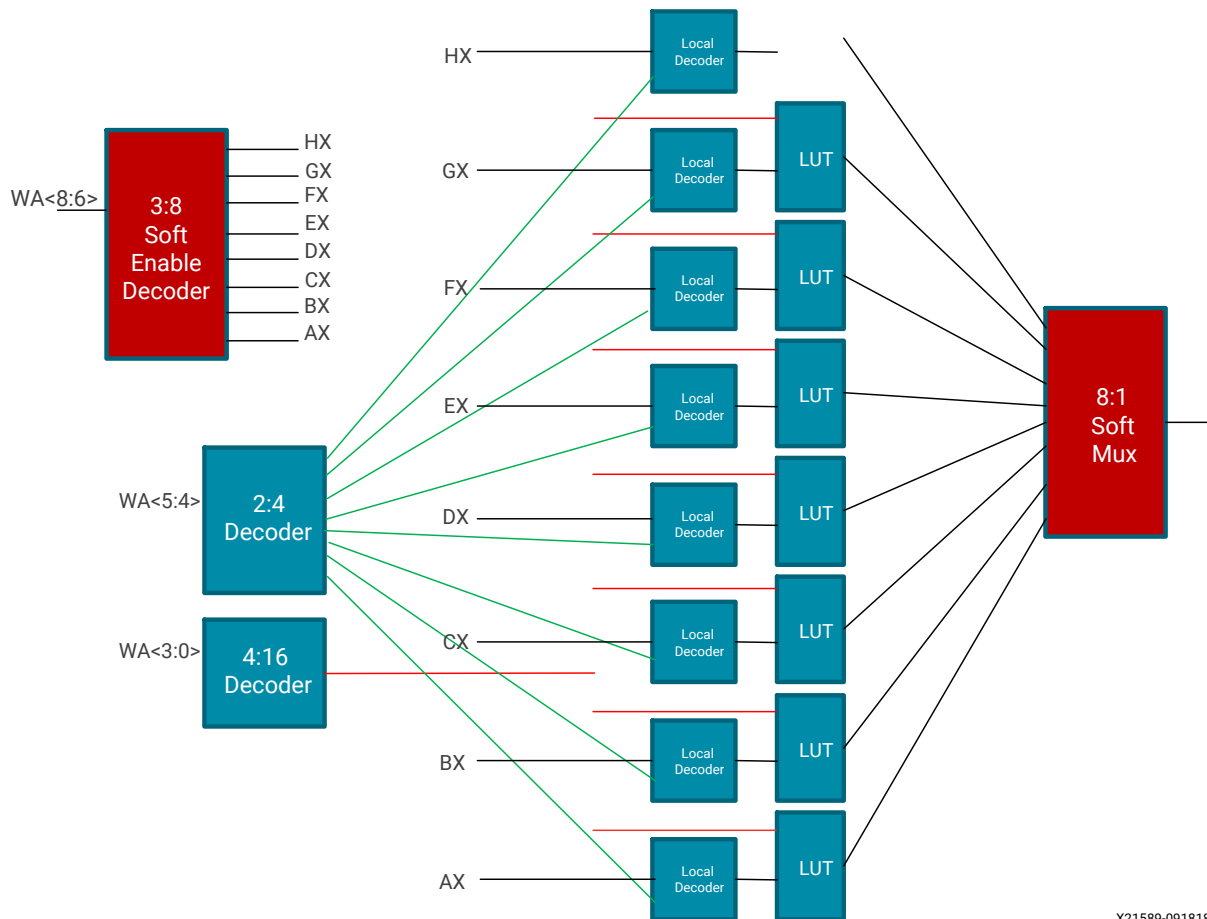
Figure 5: Write Decoder
