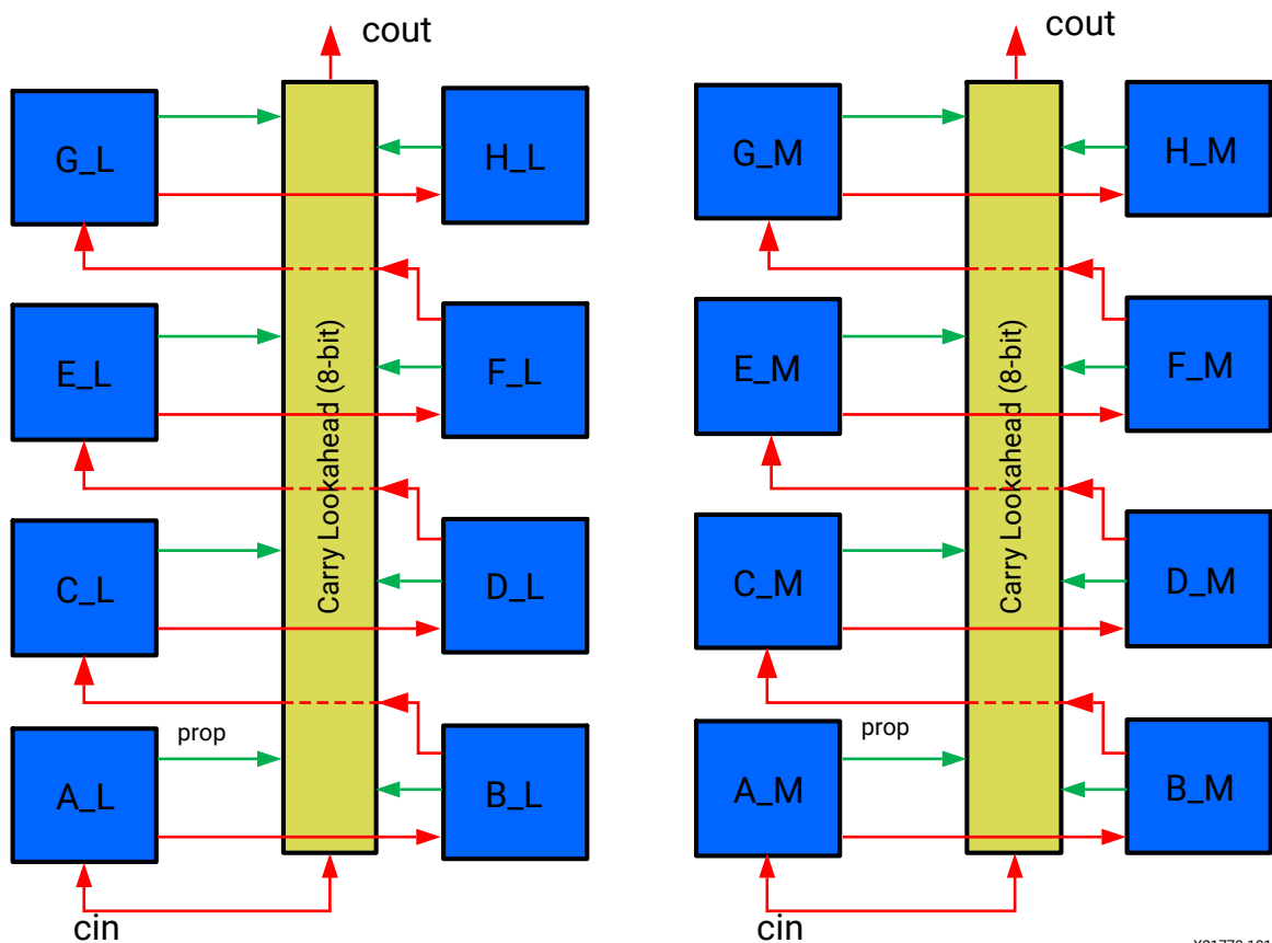
Figure 4: Cascade Pattern
