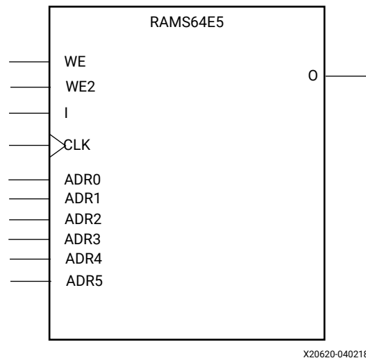
Figure 11: RAMS64E5 Distributed RAM Primitive (Single-Port)
