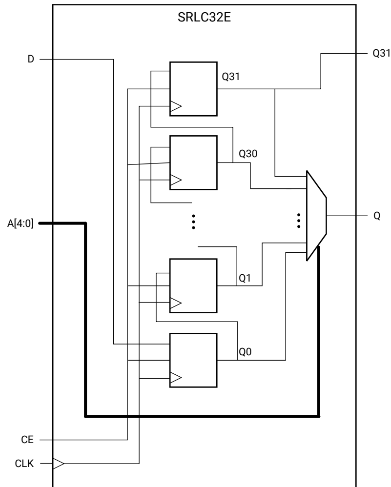
Figure 10: SRL Shift Register Primitive
