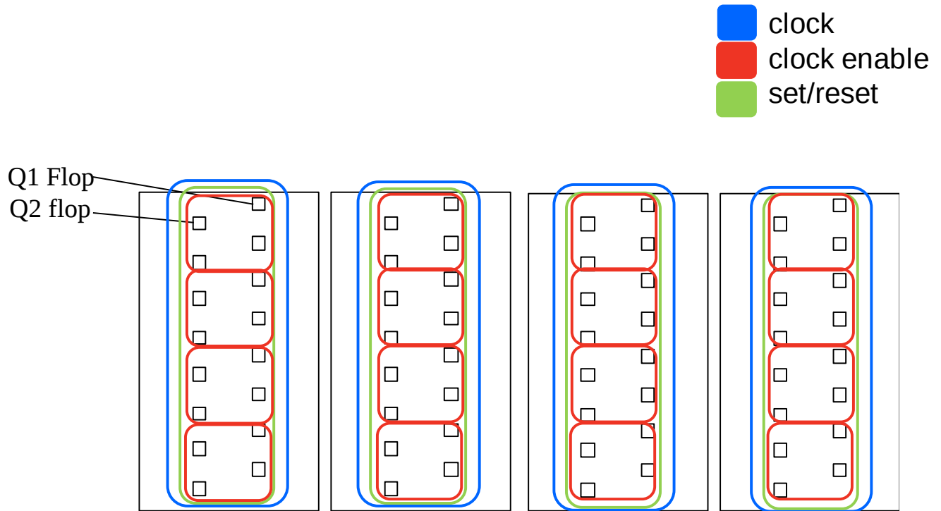
Figure 7: Control Signals
